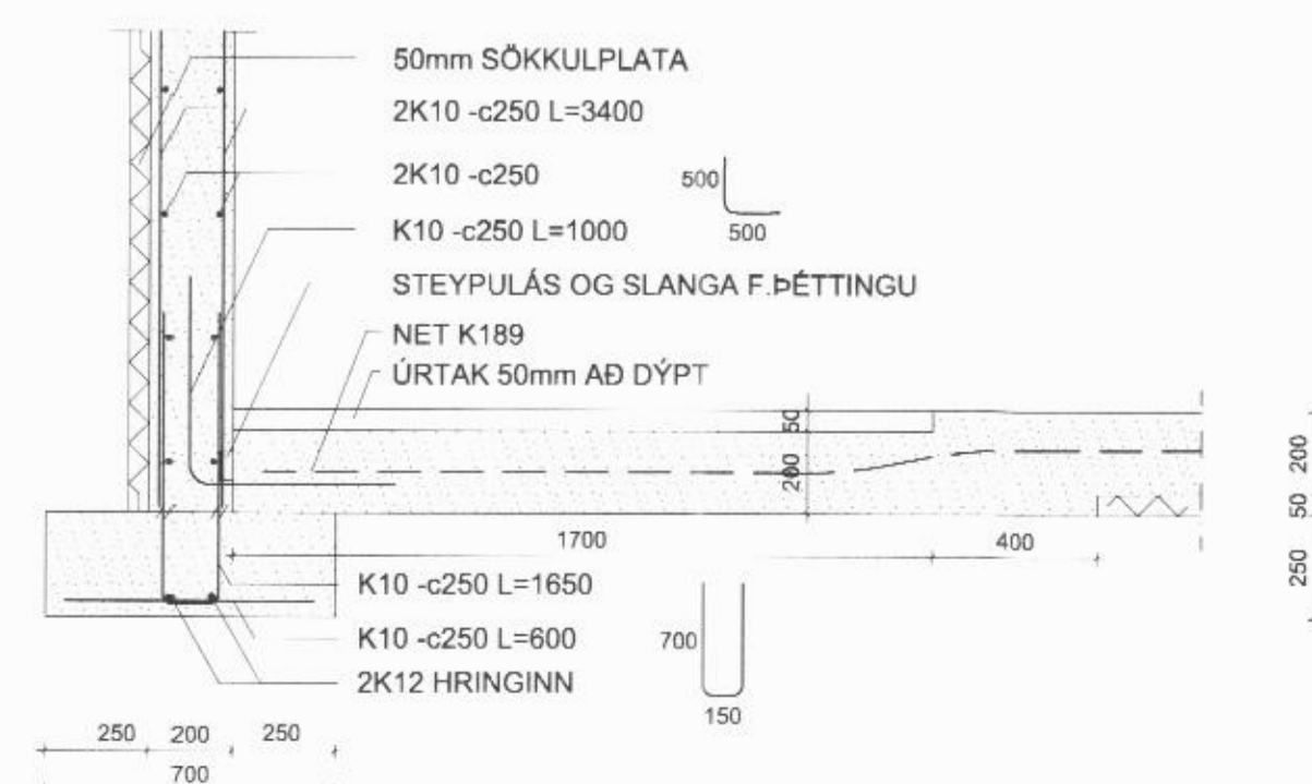
SNID 3-3 MKV.1:20
