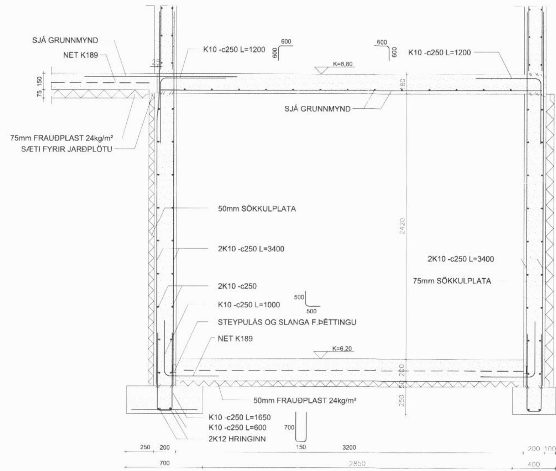
SNID 1-1 MKV.1:20
