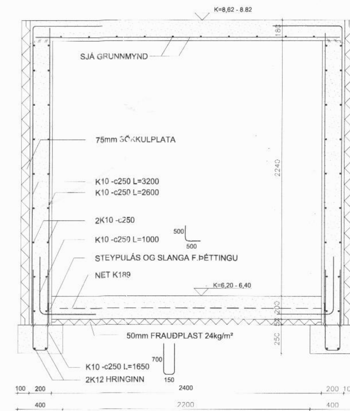
SNID 2-2 MKV.1:20
