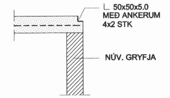
SNID 4-4 MKV. 1:20
