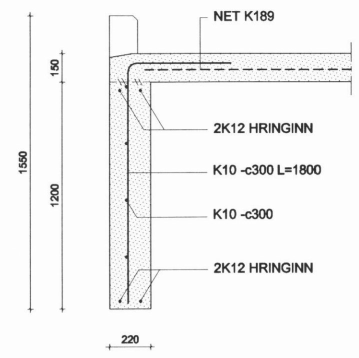
SNID 2-2 MKV. 1:20
