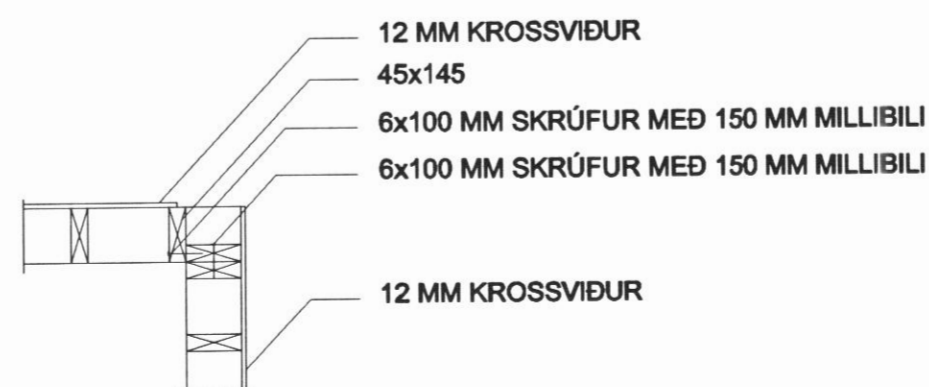
HORN MKV.1:20
