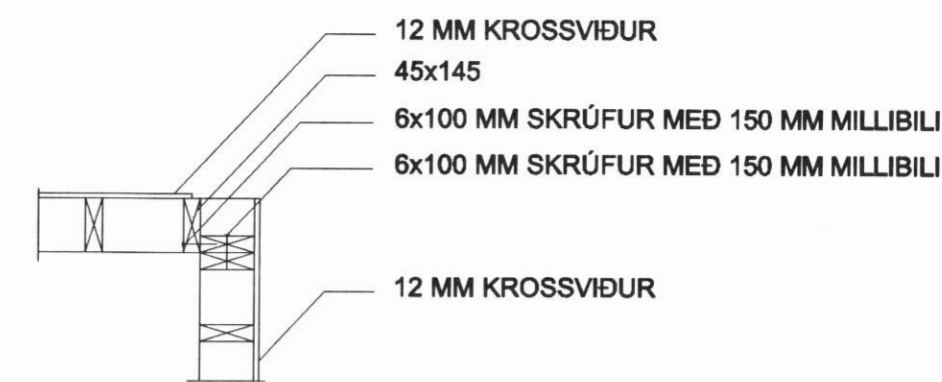
HORN MKV.1:20
