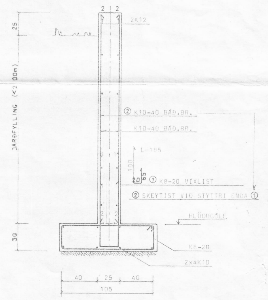
SNID B - B M=1:20
