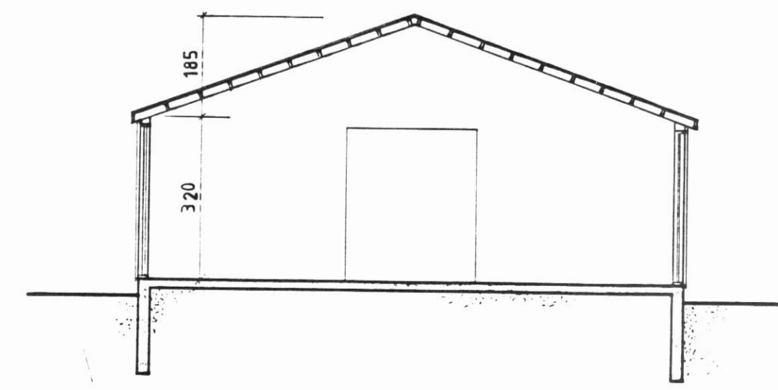
Snid C-C
