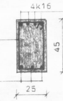
SNID B 2 - B 2 M = 1:20
