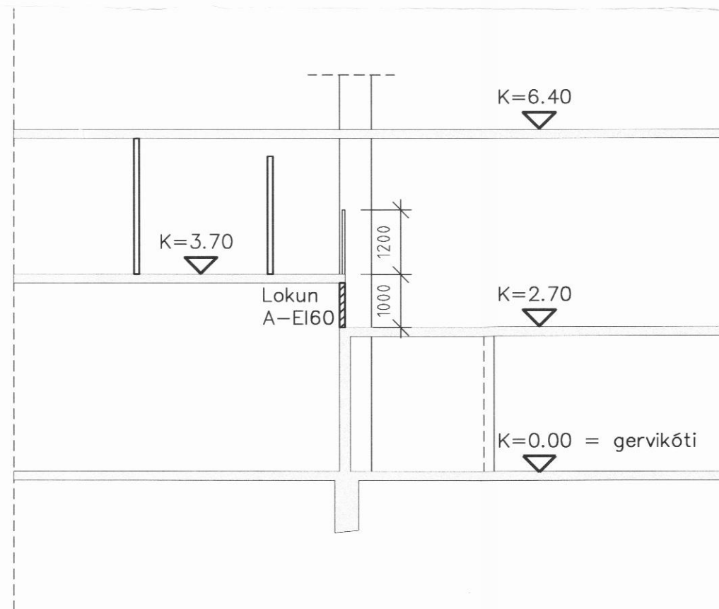
SNID b-b
