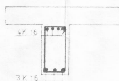
SNID B B M=1:20
