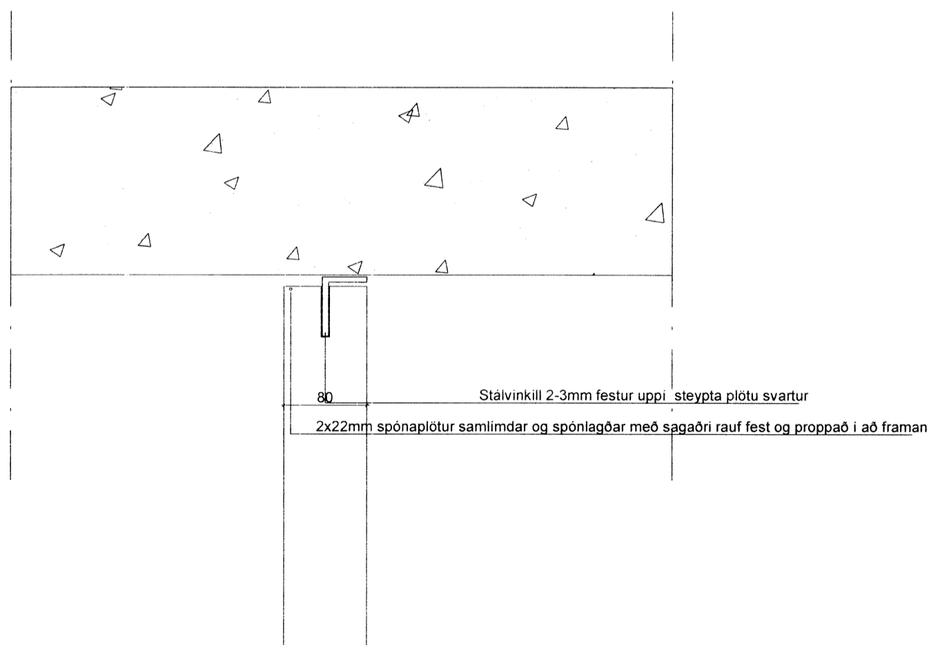
Stigadeili 1
