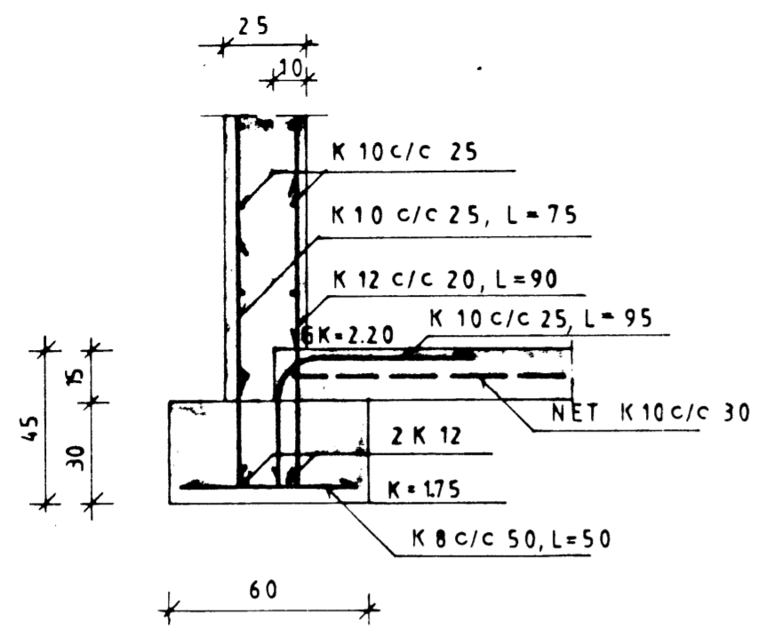
SNID 4-4, 1:20
