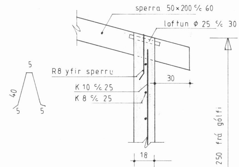
SN1Ð 2-2 Mkv. 1:20
