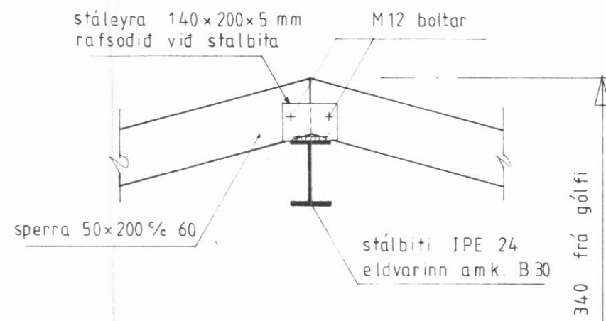
SN1Ð 1-1 Mkv. 1:20
