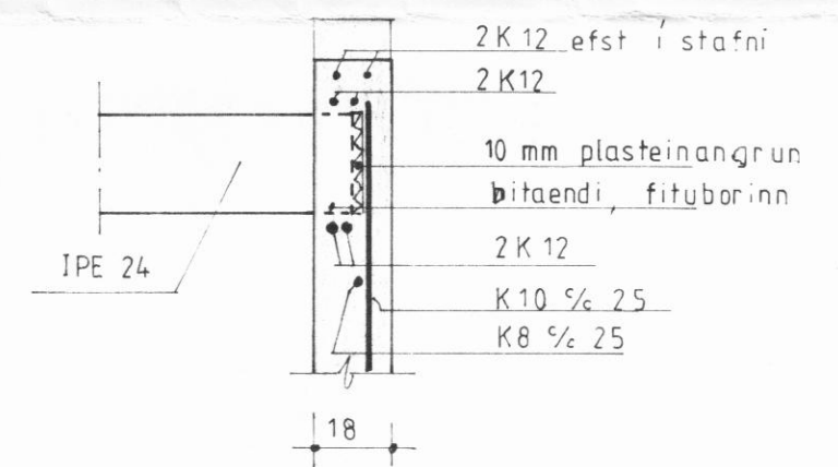
SN1Ð 4-4 Mkv. 1:20
