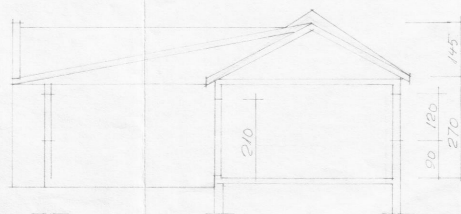
SNID B-B
