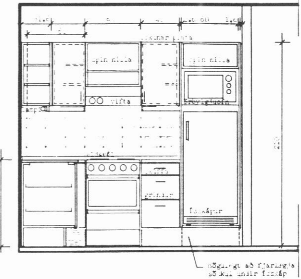
SNID B-B
