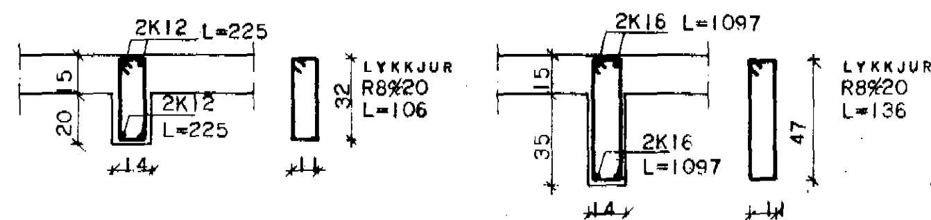
SNIB C-C 1:20
