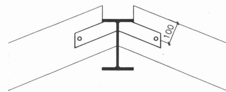
SNID Q 1:10
