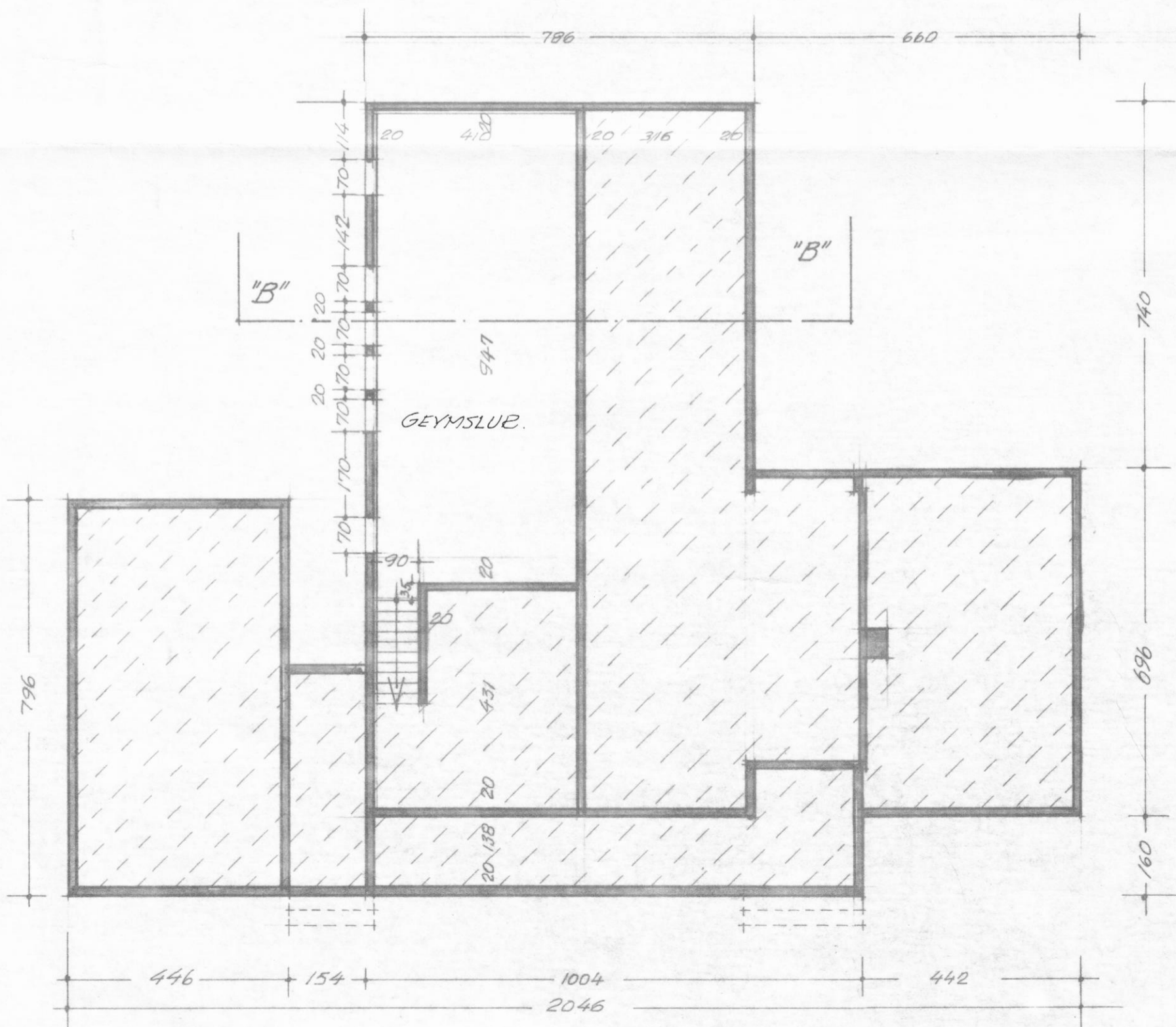
GRUNNPLAN : KJALLARI
