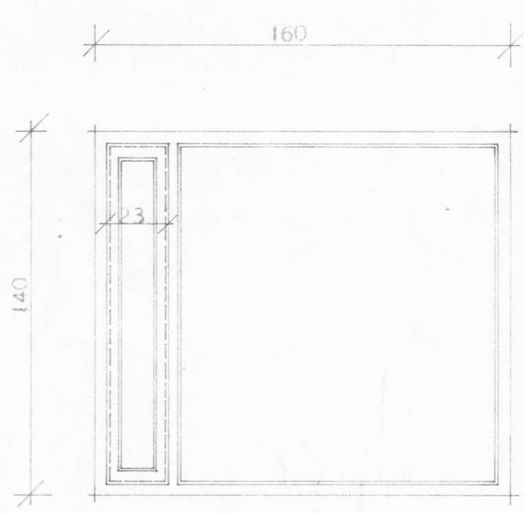
7 STK. HERBERGISGLUGGAR.
