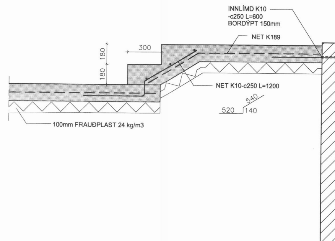
SNID 2-2 MKV. 1:20
