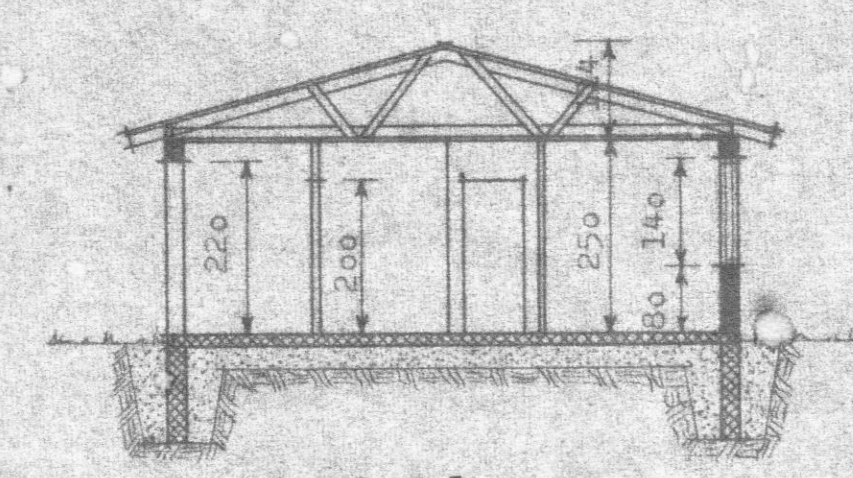
Snit C - C, 1:100
