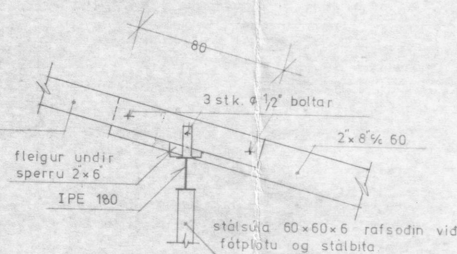
SNID 19-19, mkv. 1:20
