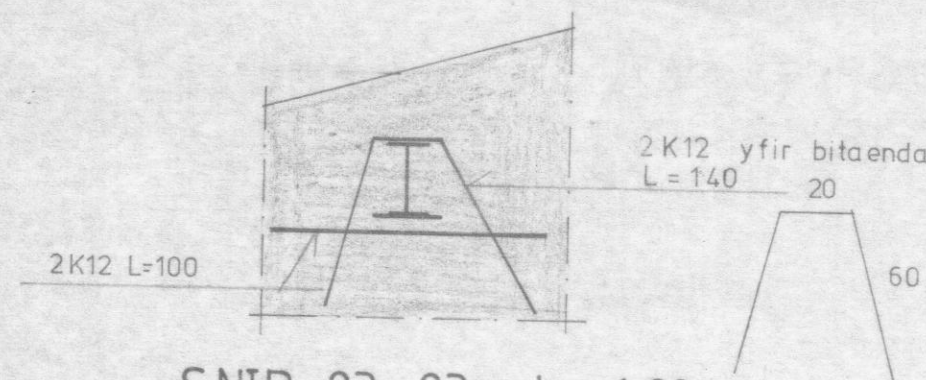
SNID 23-23 mkv. 1:20
